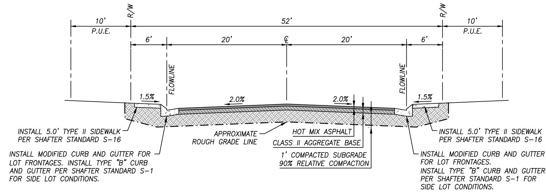
C LOCAL STREET
