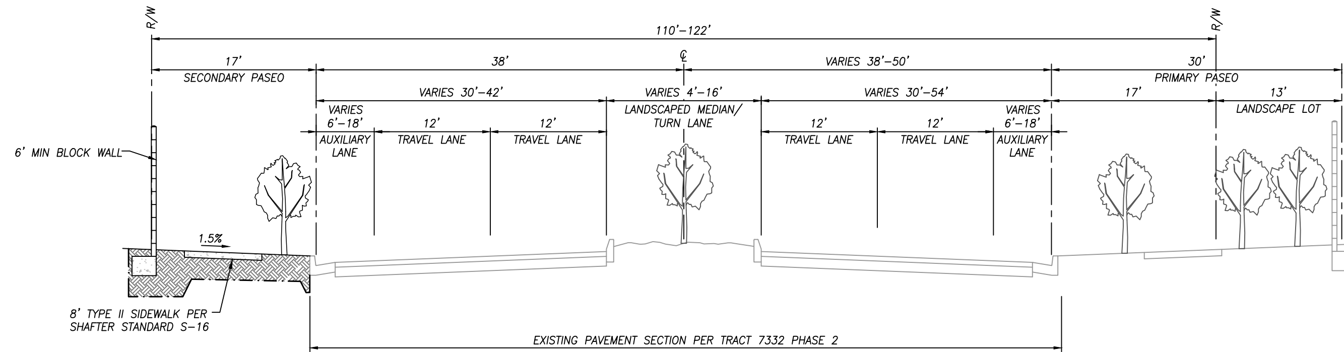
A 2 GOSSAMER GROVE BOULEVARD LOOKING NORTH NTS
