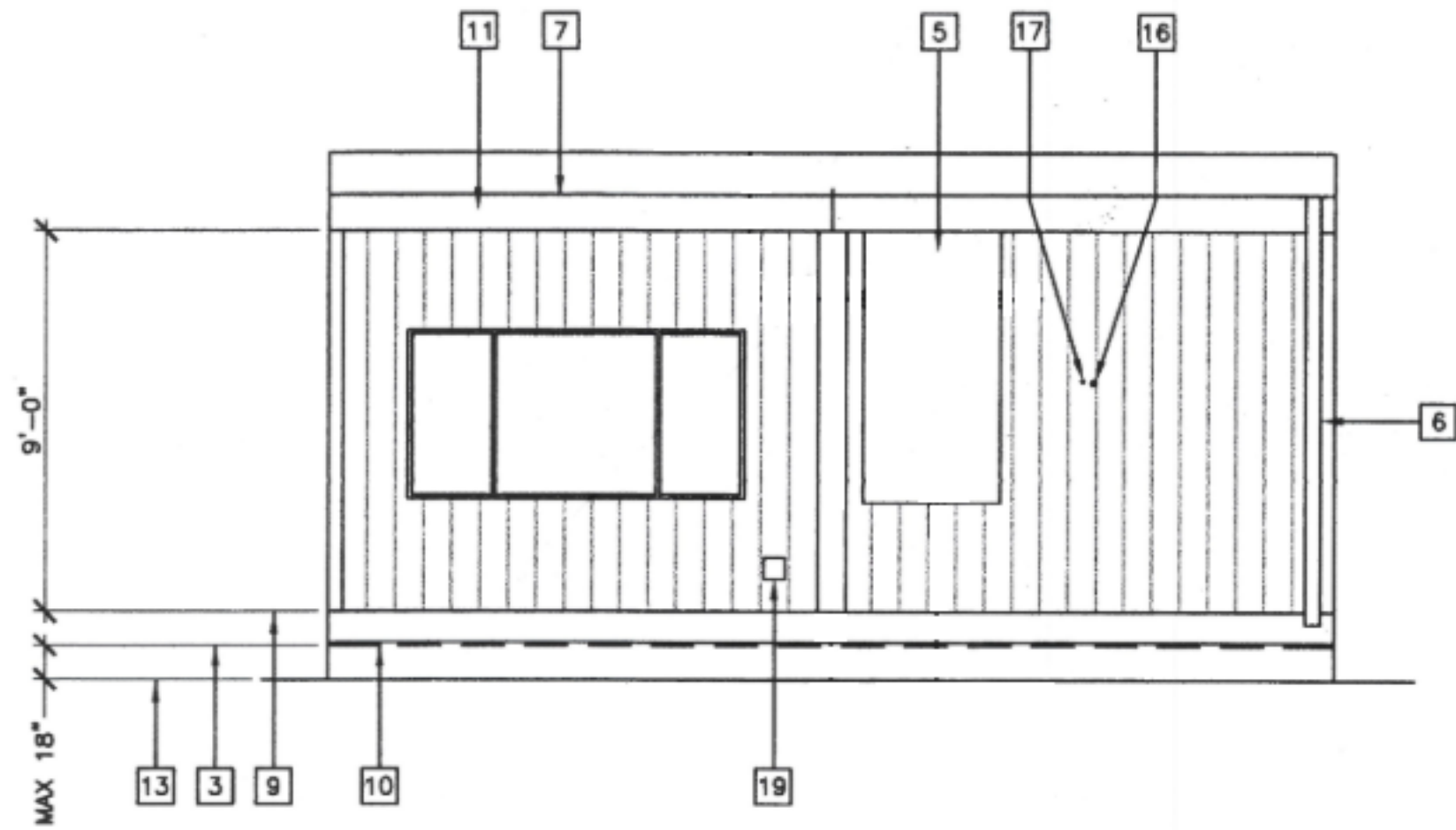
3 REAR ELEVATION
