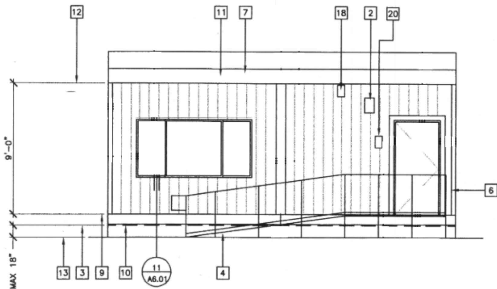
2 FRONT ELEVATION
