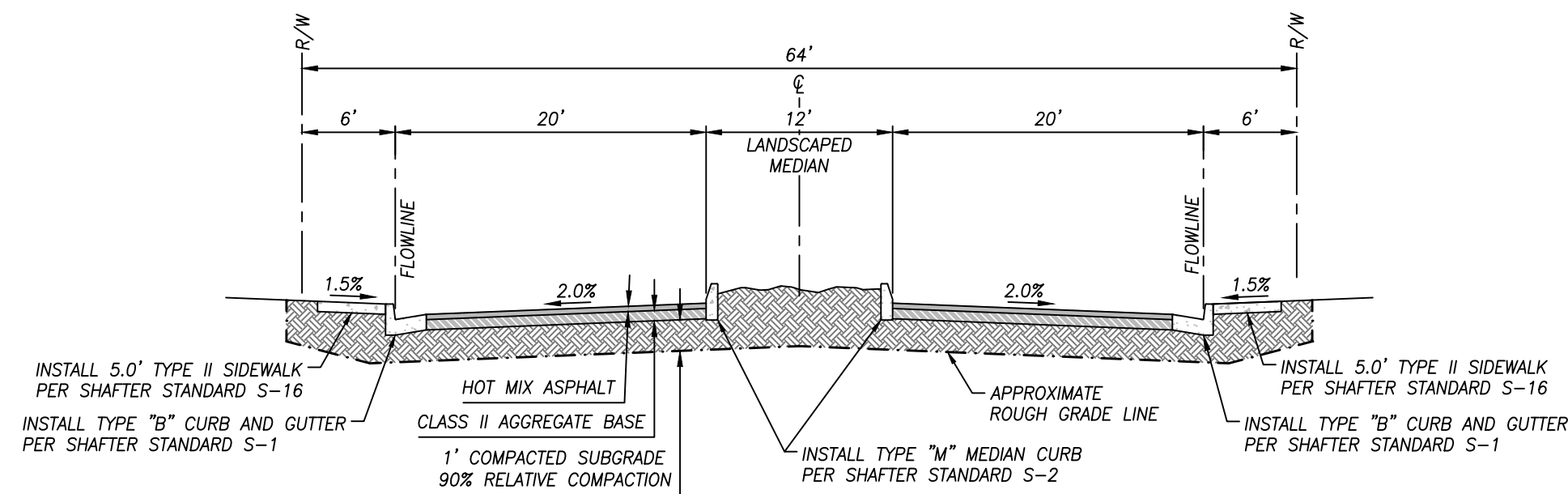
LOCAL STREET (WITH 12' MEDIAN)
